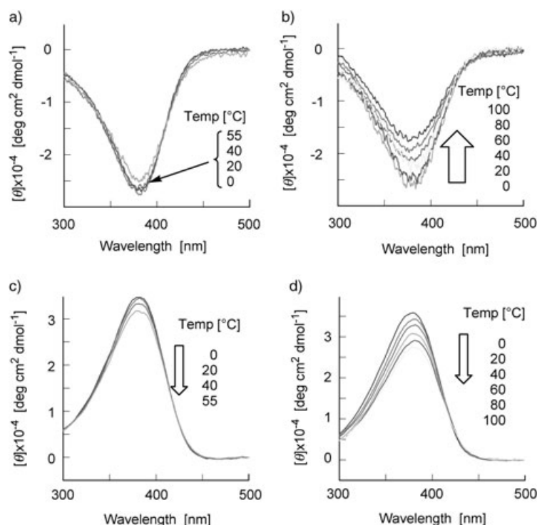
Figure 2. Variable-temperature CD spectra of poly(1), measured in a) CHCl 3 and b) toluene; and of poly(2), measured in c) CHCl 3 and d) toluene ( c = 0.084\text{--}0.19 \text{ mm} ).
