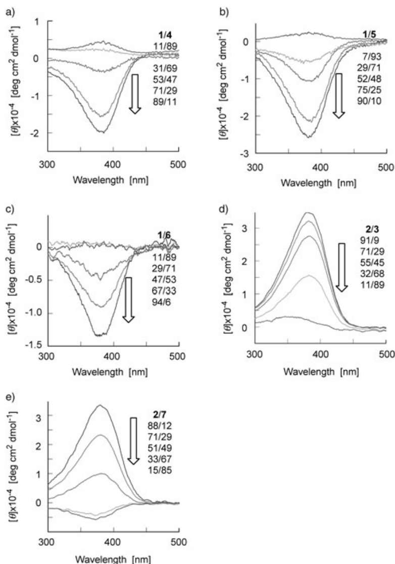
Figure 4. CD spectra of poly( 1-co-4 ), poly( 1-co-5 ), poly( 1-co-6 ), poly( 2-co-3 ), and poly( 2-co-7 ) (a)–(e), respectively, measured in \text{CHCl}_3 at 20 °C ( c = 0.072\text{--}0.14 mm).
