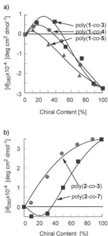
Figure 5. Molar ellipticities at 380 nm, measured in CHCl 3 at 20 °C, versus chiral content of a) poly(1-co-3), poly(1-co-4), and poly(1-co-5); and b) poly(2-co-3) and poly(2-co-7).
