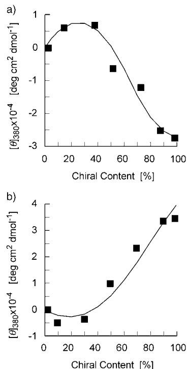
Figure 6. Chiral contents versus [\theta]_{380} of a) poly(1-co-3) and b) poly(2-co-7), measured in CHCl 3 at 20 °C. ■: observed data; solid curves: theoretical values calculated with the parameters from Table 2.
