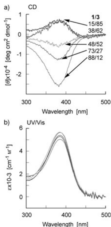
Figure 3. CD and UV/Vis spectra of poly( 1-co-3 ), measured in CHCl 3 at 20 °C ( c = 0.11\text{--}0.15 \text{ mm} ).
