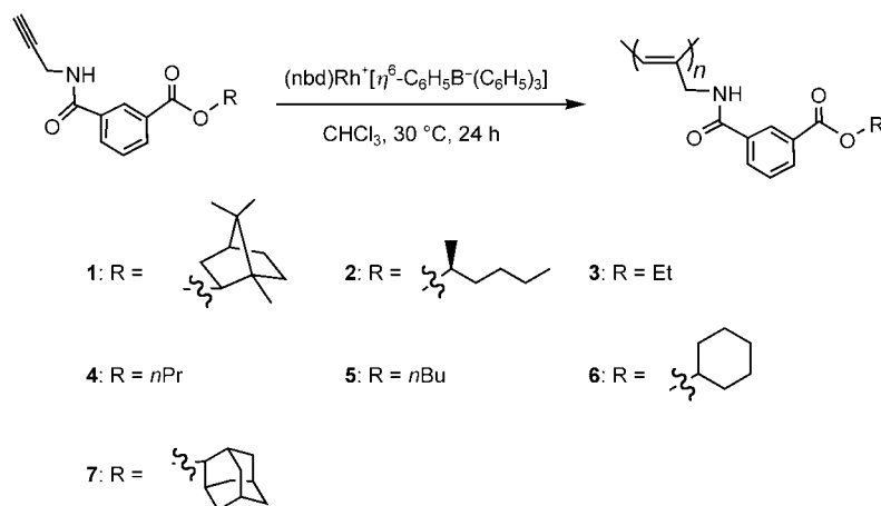
Scheme 1. Rhodium-catalyzed copolymerization of chiral and achiral N -propargylbenzamides 1–7 .
