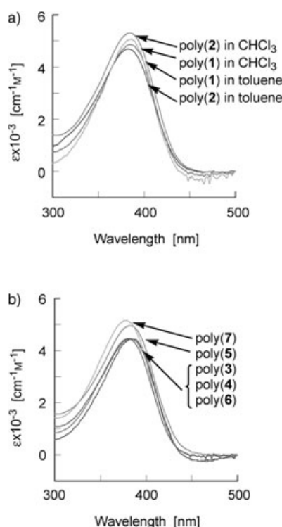
Figure 1. UV/Vis spectra of a) poly(1) and poly(2), measured in CHCl 3 and in toluene, and b) poly(3)–poly(7), measured in CHCl 3 at 20 °C ( c = 0.074\text{--}0.19 \text{ mm} ).
